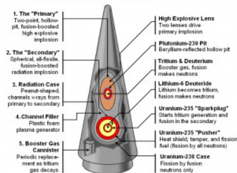
W88 Warhead for Trident D-5 Ballistic Missile
