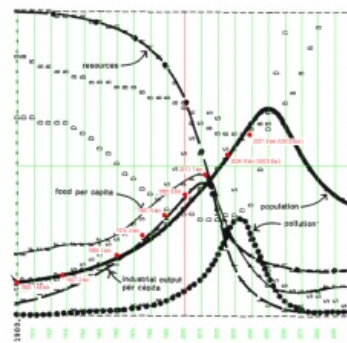
Figure 35 WORLD MODEL STANDARD RUN
