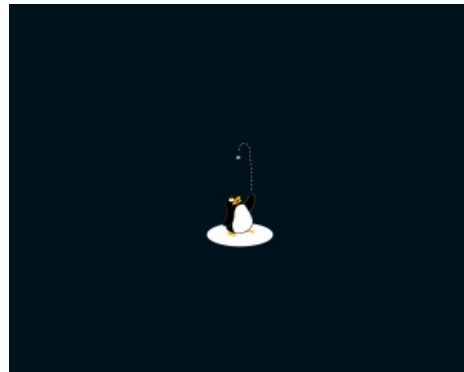
Ping localhost
